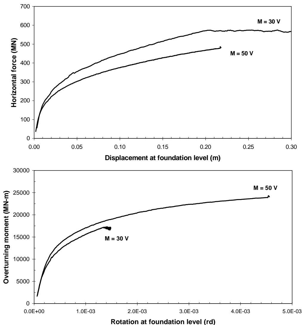
FIG. 14. Finite element analyses: force-displacement curves
