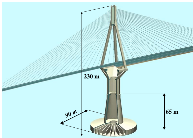
FIG. 9. View of one pylon of the Rion-Antirion bridge
