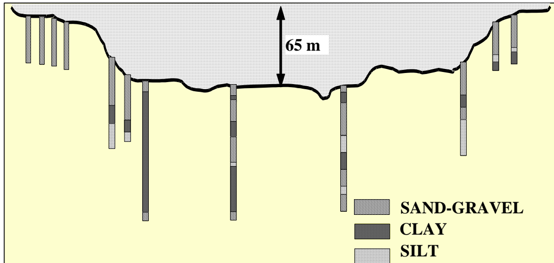
FIG. 3. Soil profile
