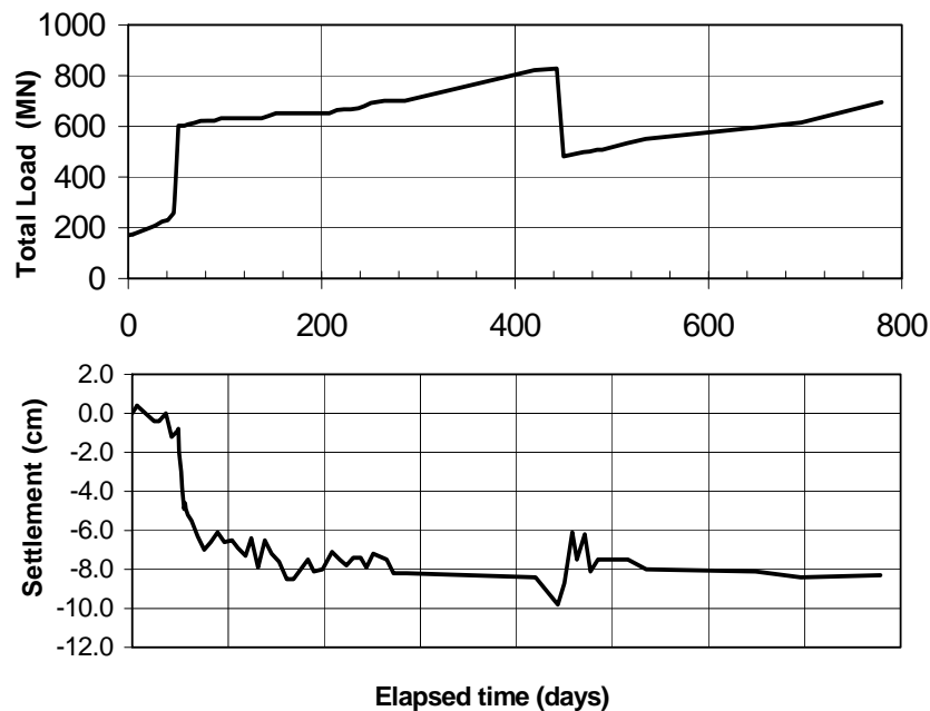
FIG. 11. Settlement versus time – Pier M3
