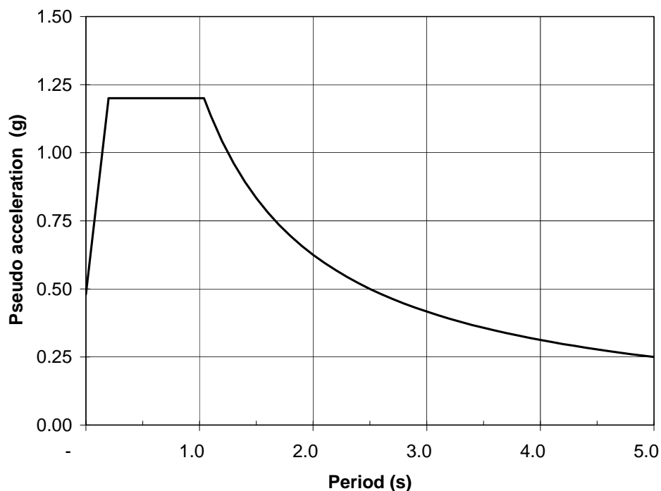
FIG. 8. Design ground surface response spectrum
