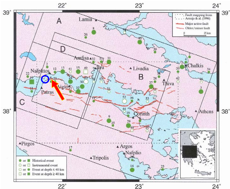
FIG. 7. Locations of major earthquakes
