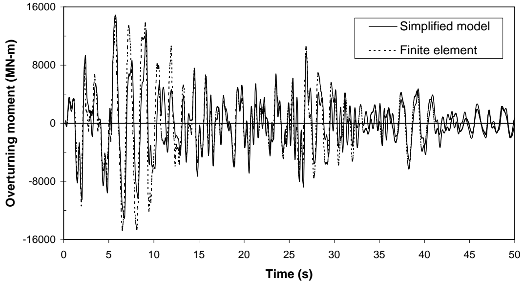
FIG. 18. Time history of foundation overturning moment
