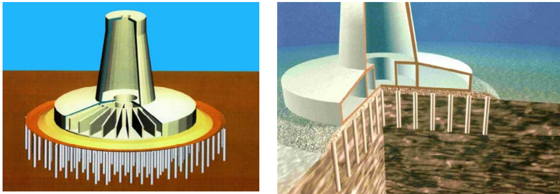
FIG. 10. Foundation reinforcement
