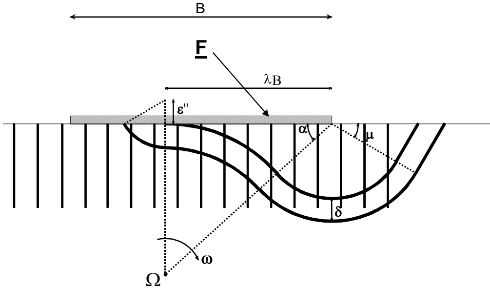
FIG. 12. Kinematic mechanism
