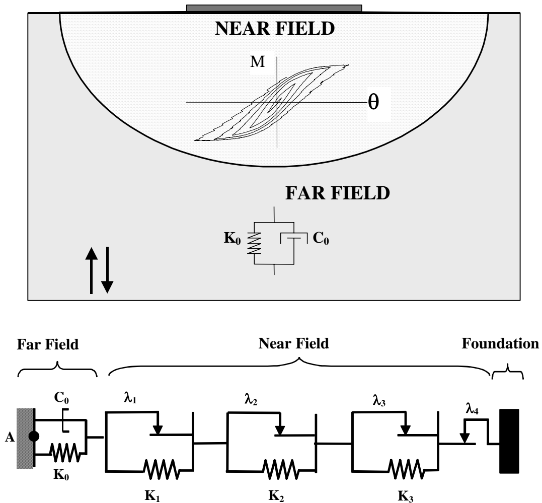
FIG. 17. Macro-element for soil structure interaction
