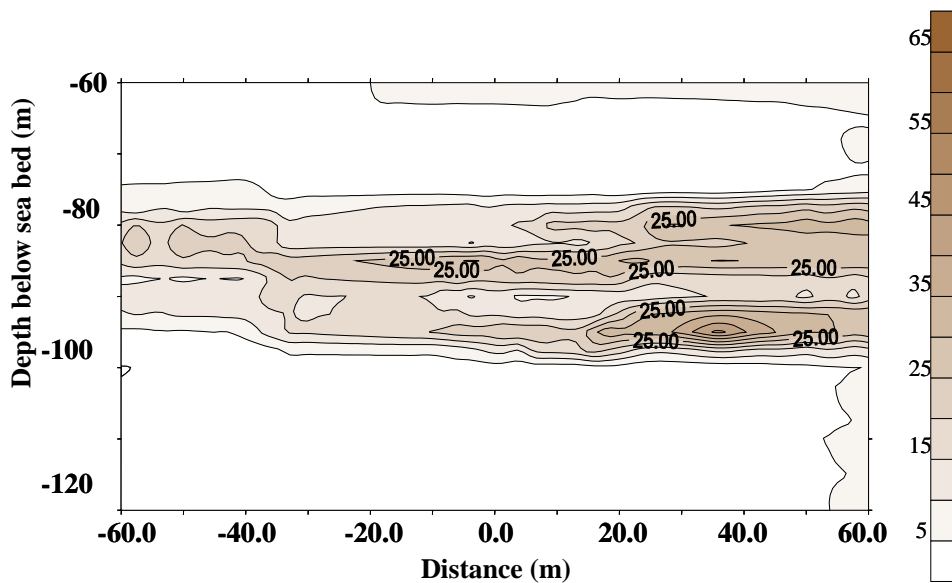
FIG. 6. Spatial variability of cone point resistance across Pier M3
