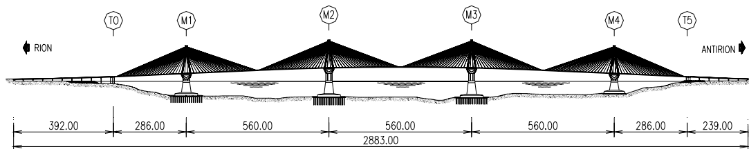
FIG. 2. Bridge elevation
