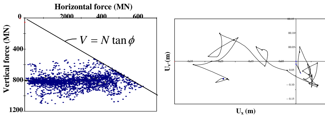
FIG. 19. Time history of foundation displacement
