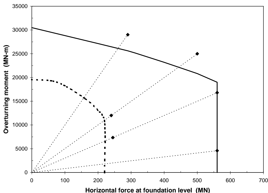
FIG. 13. Cross section of the bounding surface: Dotted line without inclusions; solid line with inclusions
